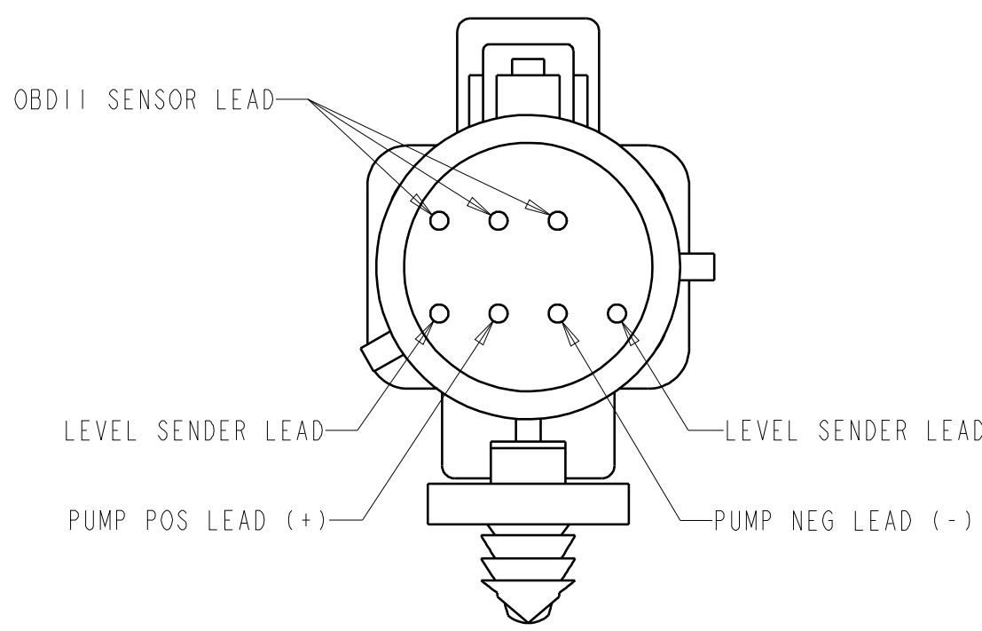
CONNECTOR MODULE MAIN PINOUT DETAIL SCALE 2:1
